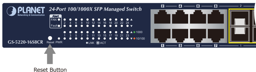
Figure 5-1: GS-5220-16S8C(R) Reset Button
